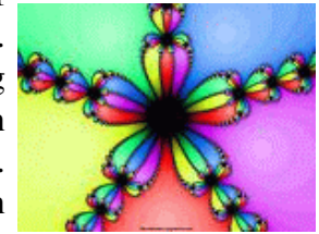
Fractals
